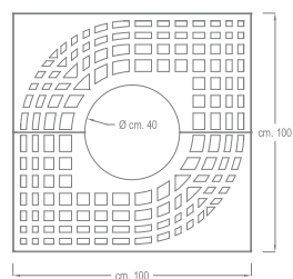
VISTA IN PIANTA / PLAN VIEW
