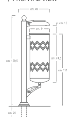
VISTA FRONTALE / FRONTAL VIEW
