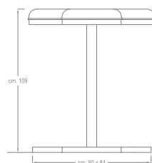
VISTA FRONTALE / FRONTAL VIEW
