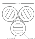
VISTA IN PIANTA / PLAN VIEW
