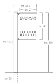
VISTA LATERALE / LATERAL VIEW
