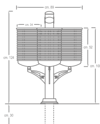
VISTA FRONTALE / FRONTAL VIEW
