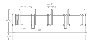
VISTA FRONTALE / FRONTAL VIEW
